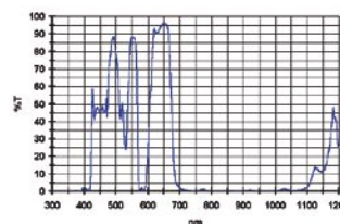
Transmission Fringe-Killer Filter & Neodymium Moon & Skyglow Filter combined
